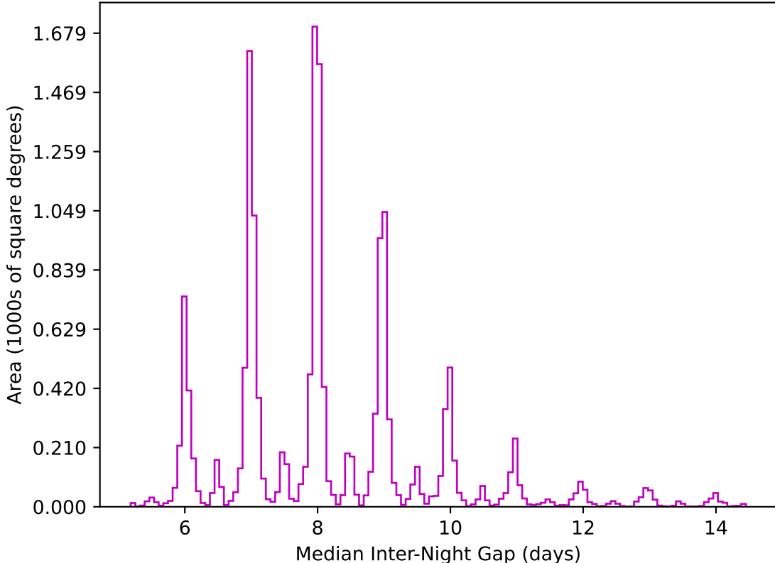
too_elab_heavy_r128_d3_griz_v3.4_10yrs WFD z band: Median Inter-Night Gap
