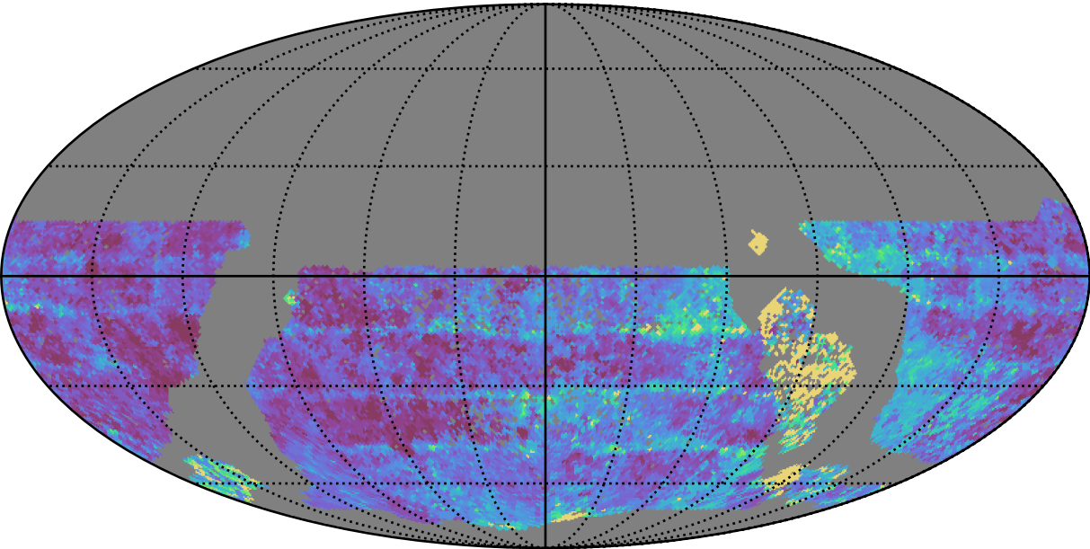
too_elab_heavy_r128_d3_griz_v3.4_10yrs WFD u band: Median Inter-Night Gap
