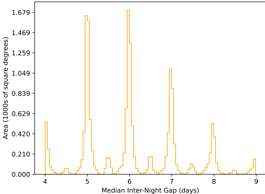
too_elab_heavy_r128_d3_griz_v3.4_10yrs WFD r band: Median Inter-Night Gap
