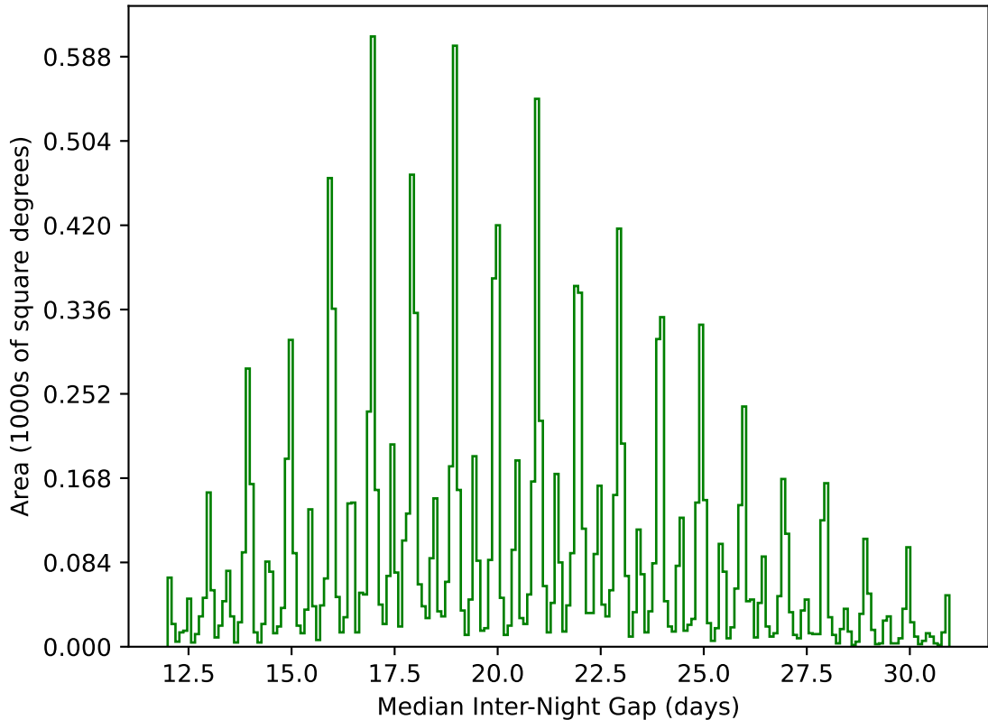
too_elab_heavy_r128_d3_griz_v3.4_10yrs WFD g band: Median Inter-Night Gap
