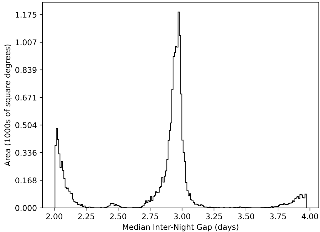
too_elab_heavy_r128_d3_griz_v3.4_10yrs WFD all bands: Median Inter-Night Gap
