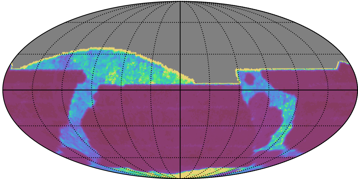
too_elab_heavy_r128_d3_griz_v3.4_10yrs All sky all bands: Median Inter-Night Gap
