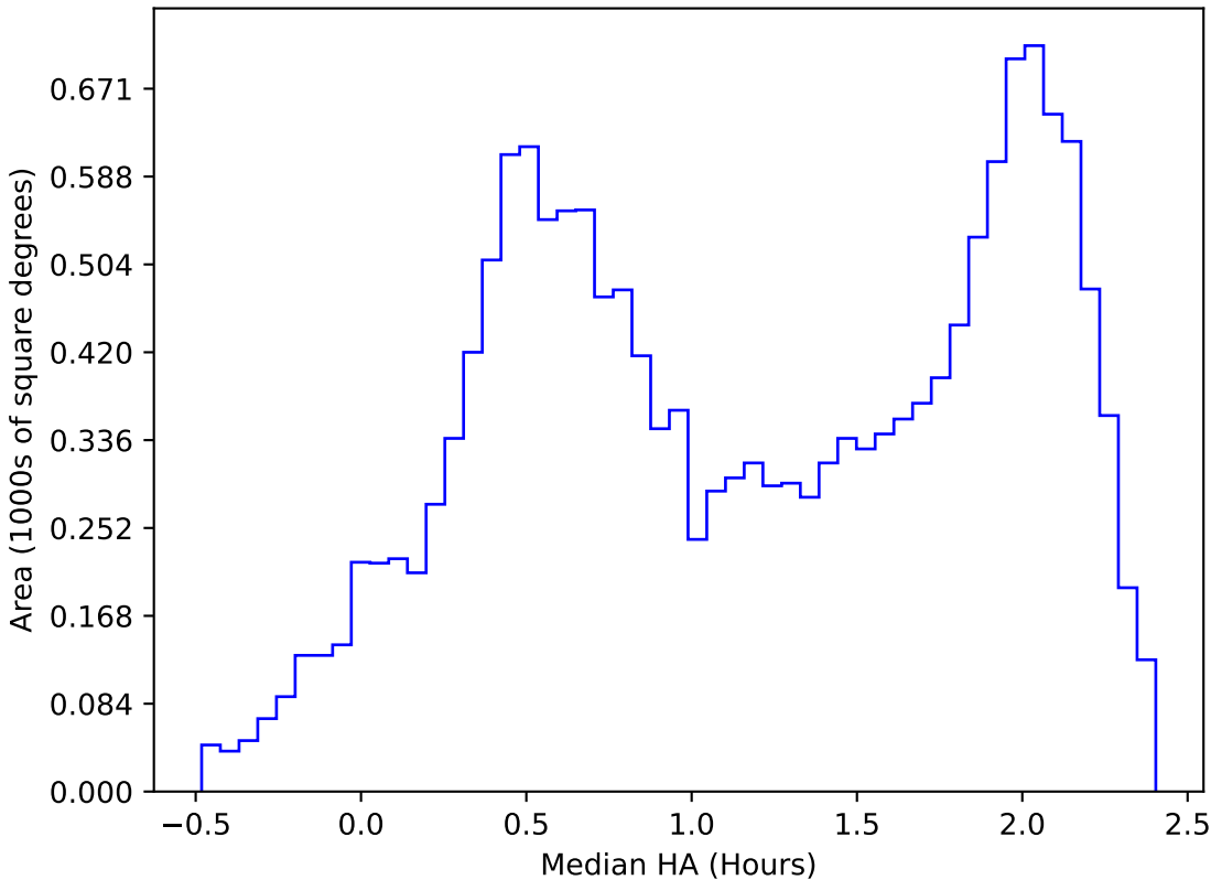
too_elab_heavy_r128_d3_griz_v3.4_10yrs WFD z band: Median HA
