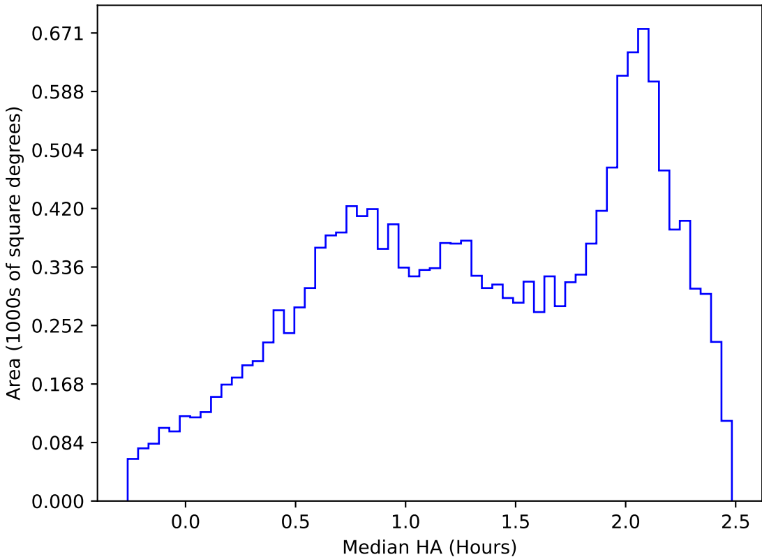
too_elab_heavy_r128_d3_griz_v3.4_10yrs WFD y band: Median HA
