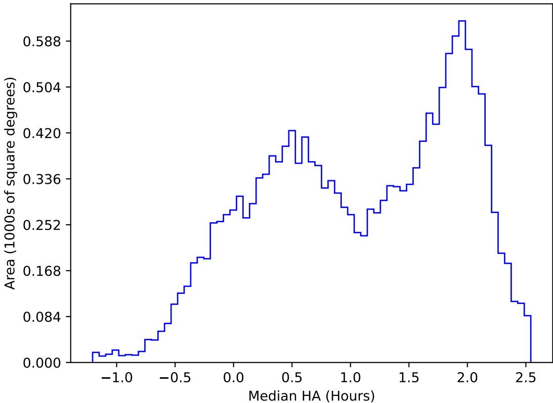
too_elab_heavy_r128_d3_griz_v3.4_10yrs WFD u band: Median HA
