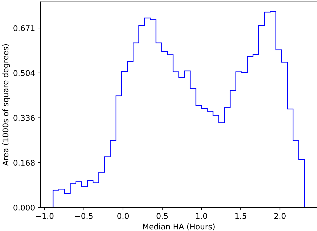
too_elab_heavy_r128_d3_griz_v3.4_10yrs WFD r band: Median HA
