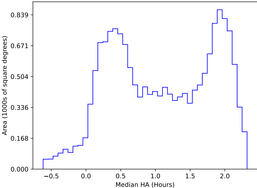
too_elab_heavy_r128_d3_griz_v3.4_10yrs WFD i band: Median HA
