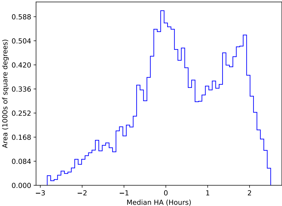
too_elab_heavy_r128_d3_griz_v3.4_10yrs WFD g band: Median HA
