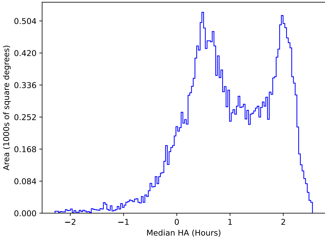
too_elab_heavy_r128_d3_griz_v3.4_10yrs All sky z band: Median HA
