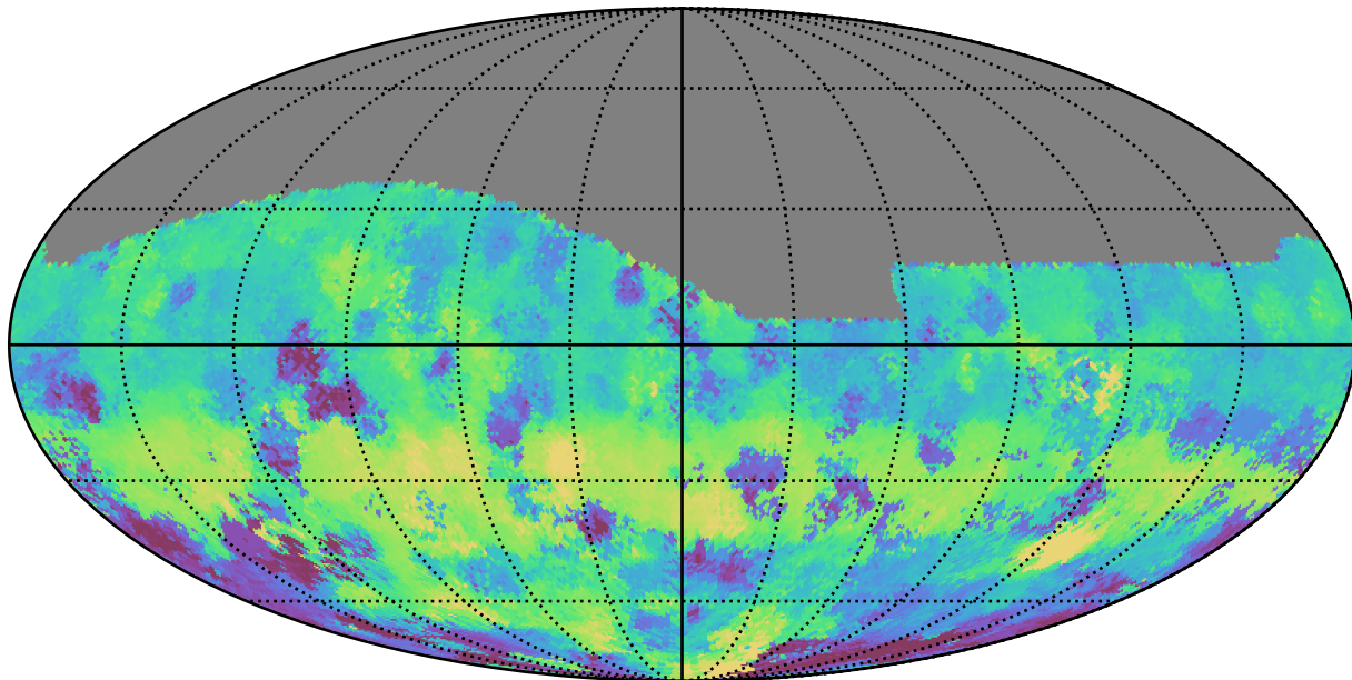
too_elab_heavy_r128_d3_griz_v3.4_10yrs All sky g band: Median HA
