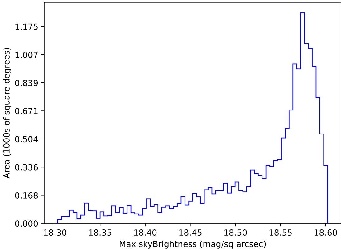
too_elab_heavy_r128_d3_griz_v3.4_10yrs WFD y band: Max skyBrightness
