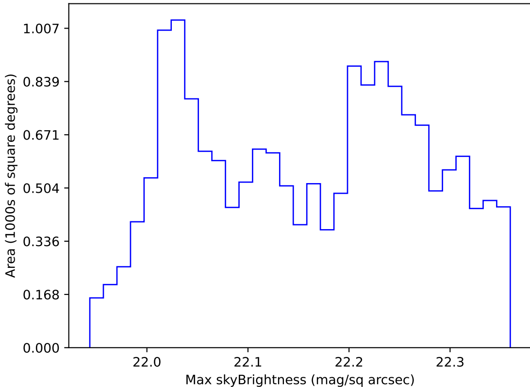
too_elab_heavy_r128_d3_griz_v3.4_10yrs WFD g band: Max skyBrightness
