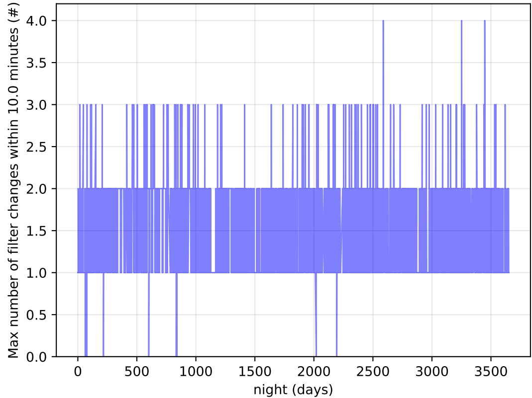
too_elab_heavy_r128_d3_griz_v3.4_10yrs Per Night: Max number of filter changes within 10.0 minutes
