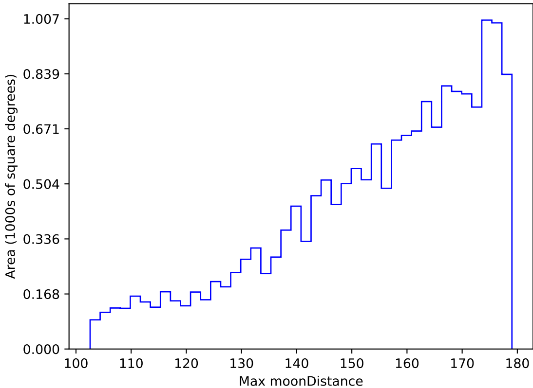
too_elab_heavy_r128_d3_griz_v3.4_10yrs WFD z band: Max moonDistance
