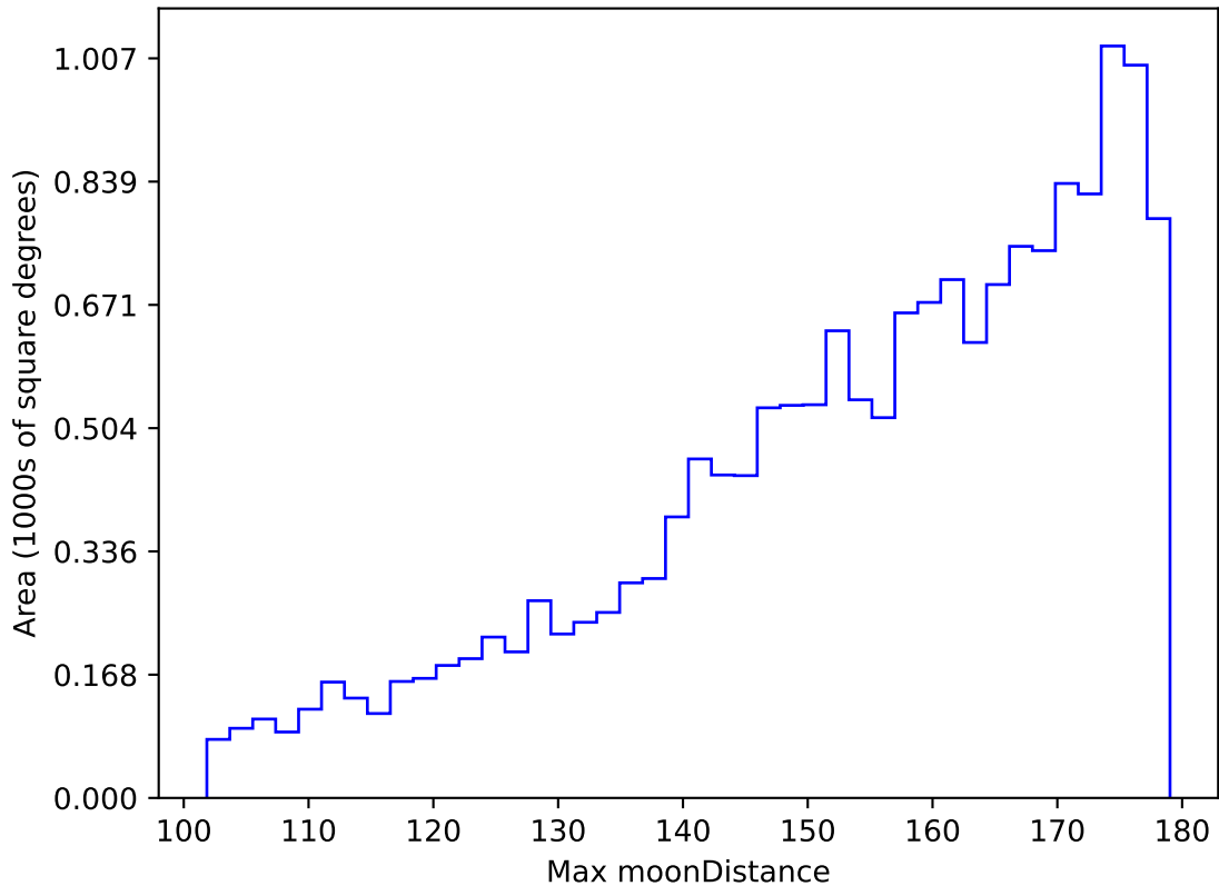
too_elab_heavy_r128_d3_griz_v3.4_10yrs WFD u band: Max moonDistance
