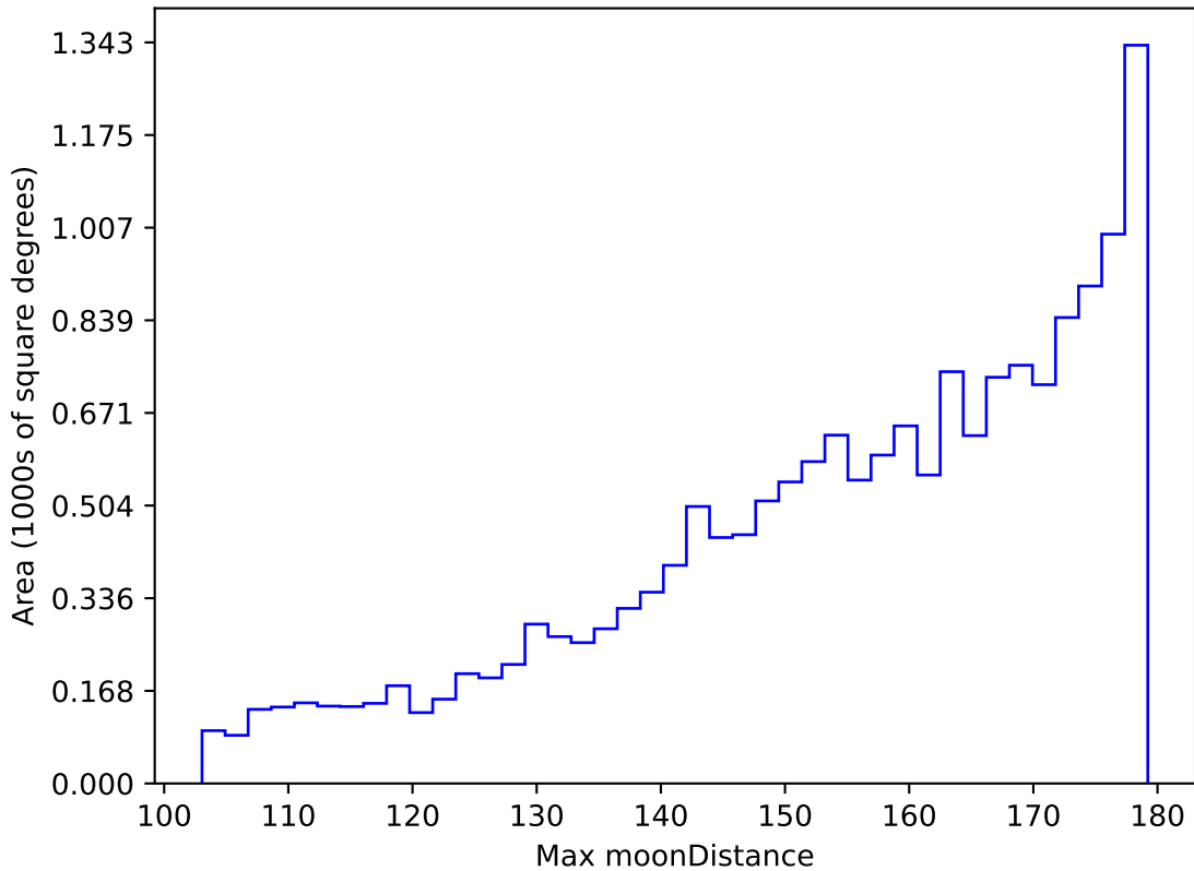
too_elab_heavy_r128_d3_griz_v3.4_10yrs WFD i band: Max moonDistance
