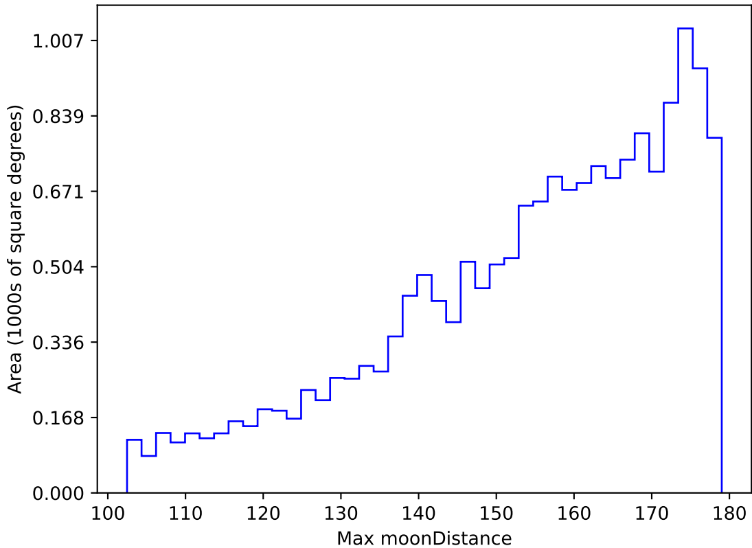
too_elab_heavy_r128_d3_griz_v3.4_10yrs WFD g band: Max moonDistance
