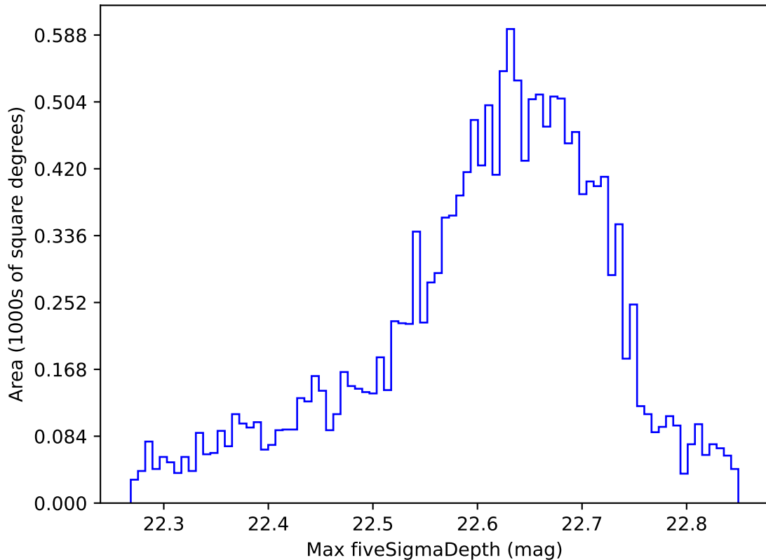
too_elab_heavy_r128_d3_griz_v3.4_10yrs WFD y band: Max fiveSigmaDepth
