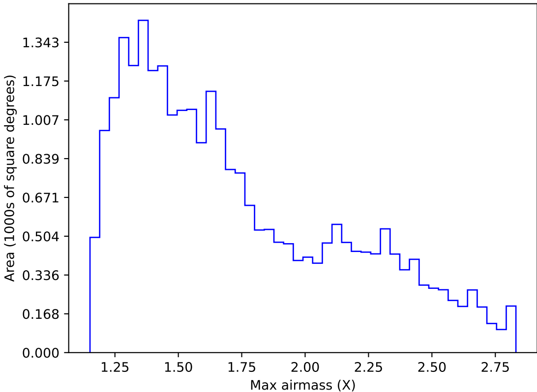
too_elab_heavy_r128_d3_griz_v3.4_10yrs Yr 1 z band: Max airmass
