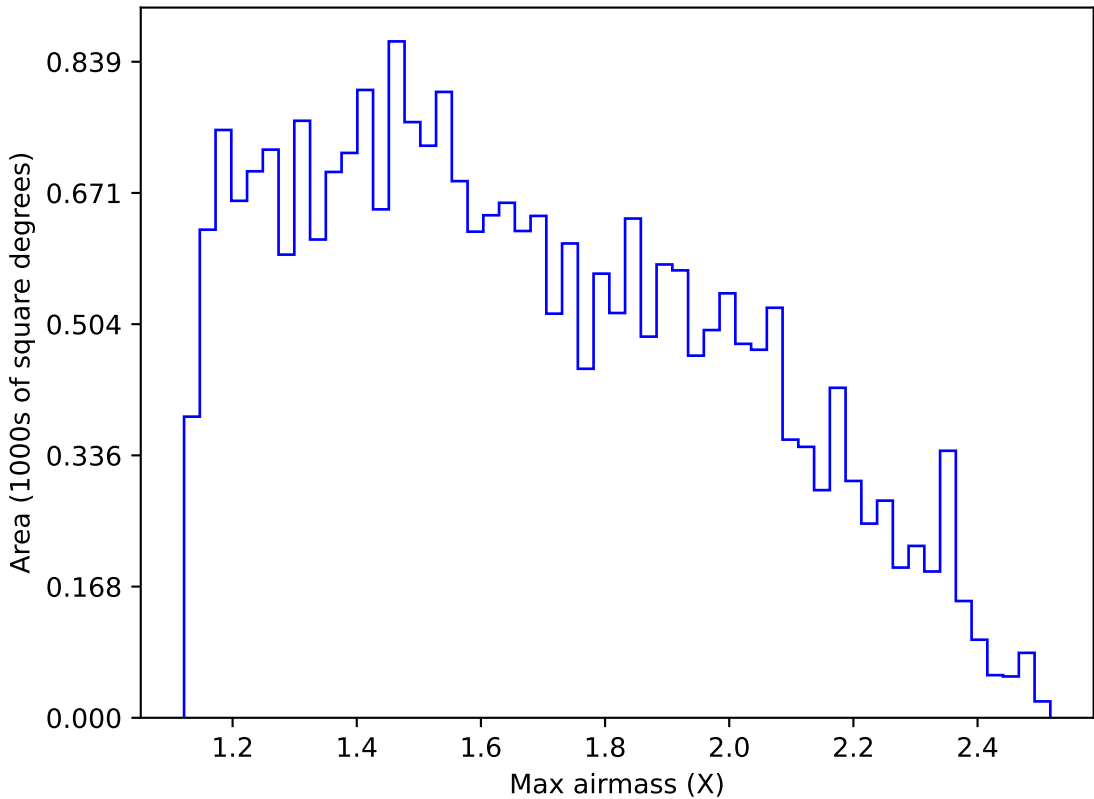
too_elab_heavy_r128_d3_griz_v3.4_10yrs Yr 1 g band: Max airmass
