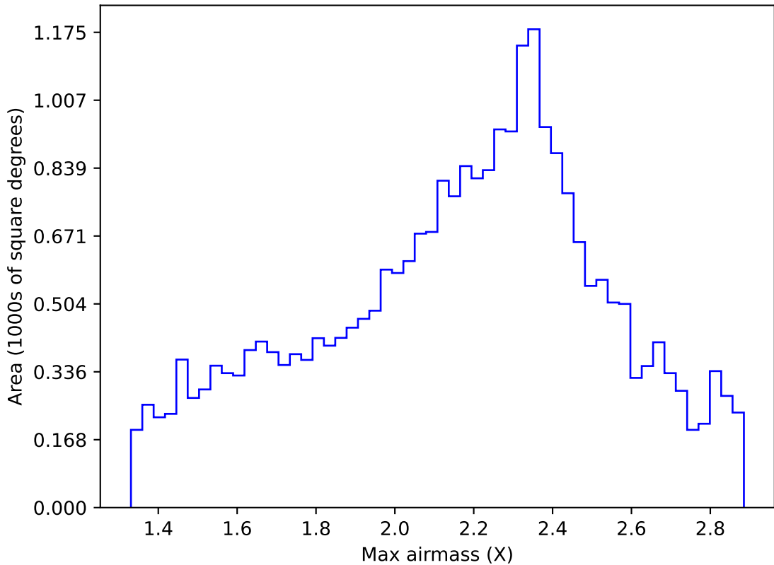
too_elab_heavy_r128_d3_griz_v3.4_10yrs Yr 1 all bands: Max airmass
