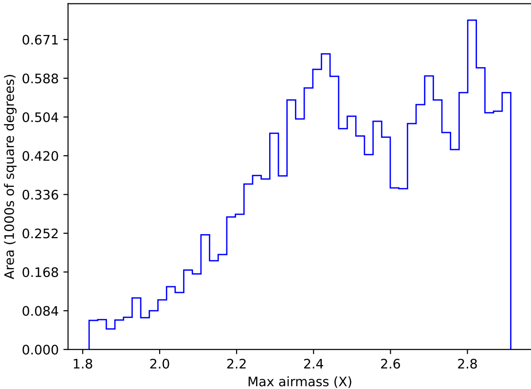
too_elab_heavy_r128_d3_griz_v3.4_10yrs WFD z band: Max airmass
