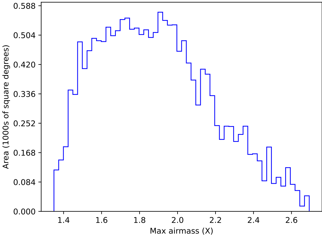
too_elab_heavy_r128_d3_griz_v3.4_10yrs WFD u band: Max airmass
