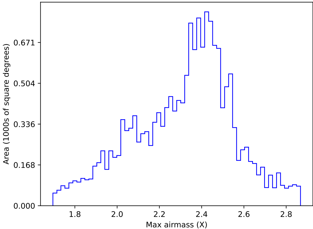
too_elab_heavy_r128_d3_griz_v3.4_10yrs WFD r band: Max airmass
