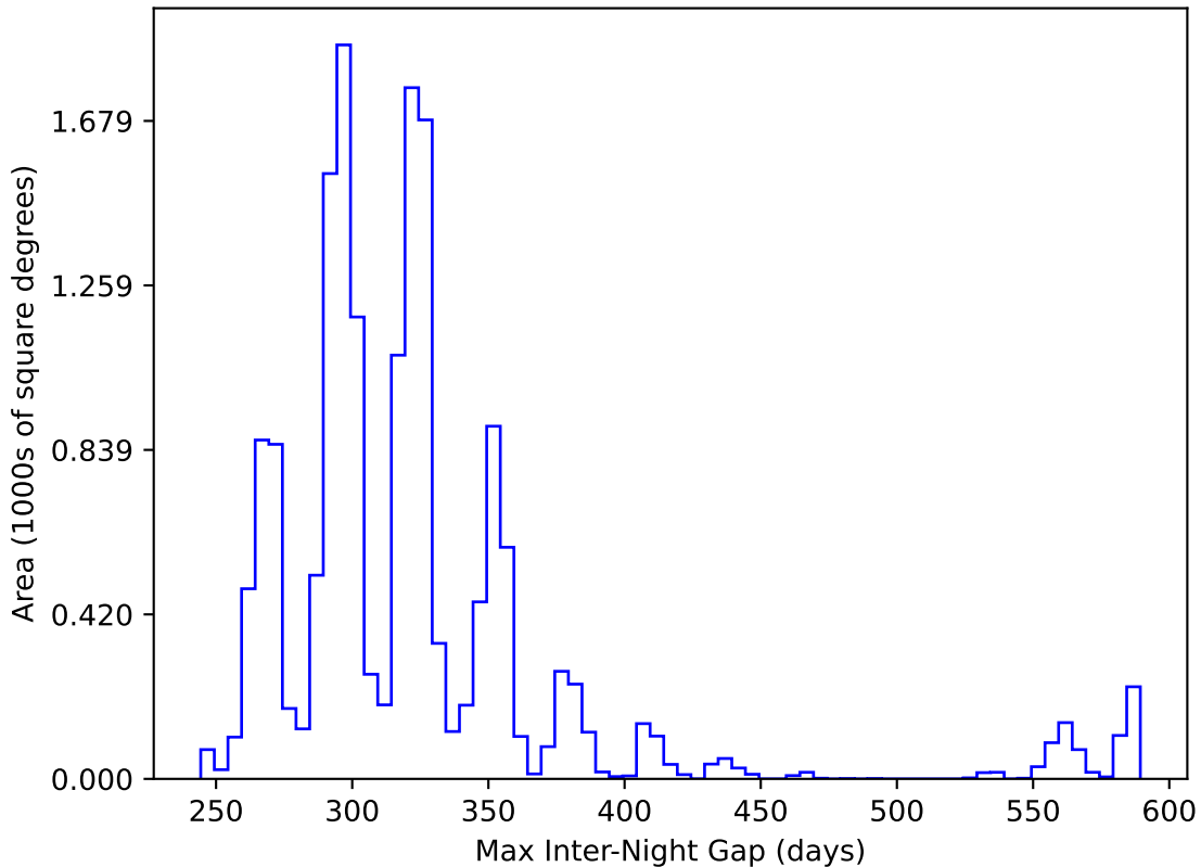
too_elab_heavy_r128_d3_griz_v3.4_10yrs WFD y band: Max Inter-Night Gap
