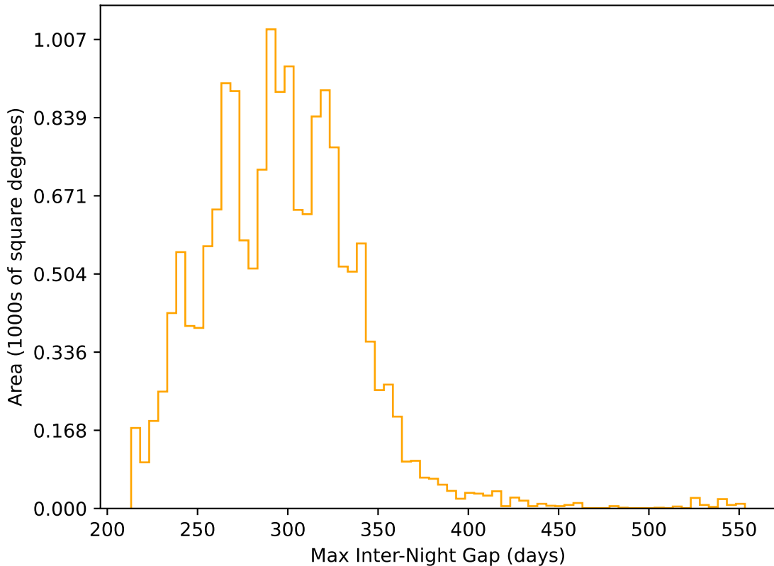
too_elab_heavy_r128_d3_griz_v3.4_10yrs WFD r band: Max Inter-Night Gap
