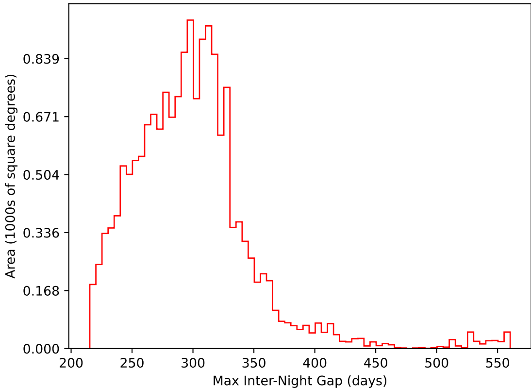
too_elab_heavy_r128_d3_griz_v3.4_10yrs WFD i band: Max Inter-Night Gap
