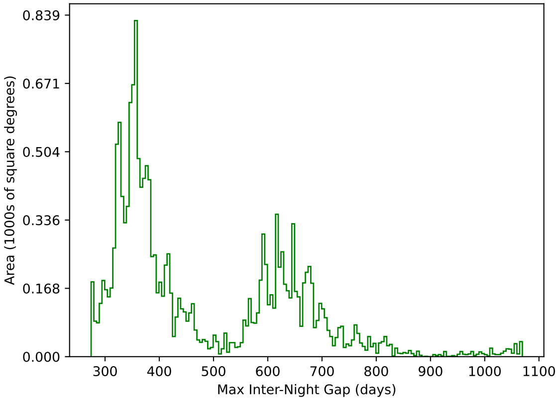
too_elab_heavy_r128_d3_griz_v3.4_10yrs WFD g band: Max Inter-Night Gap
