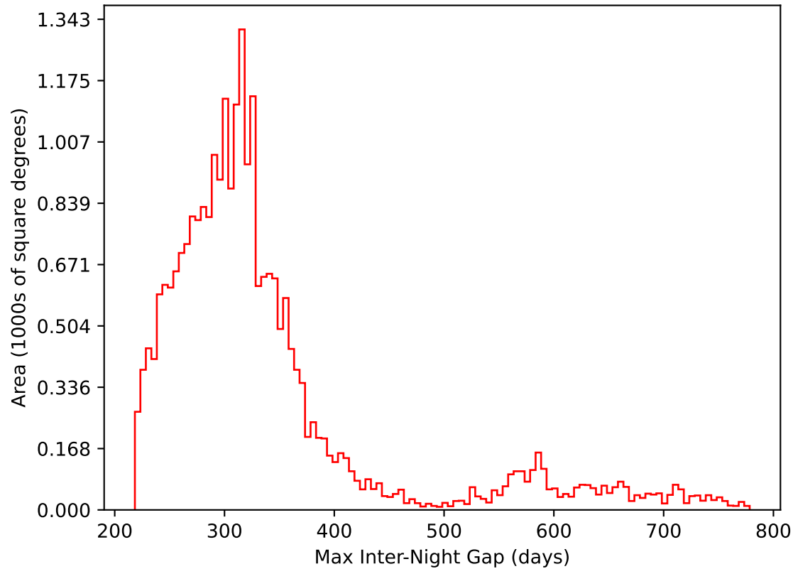
too_elab_heavy_r128_d3_griz_v3.4_10yrs All sky i band: Max Inter-Night Gap
