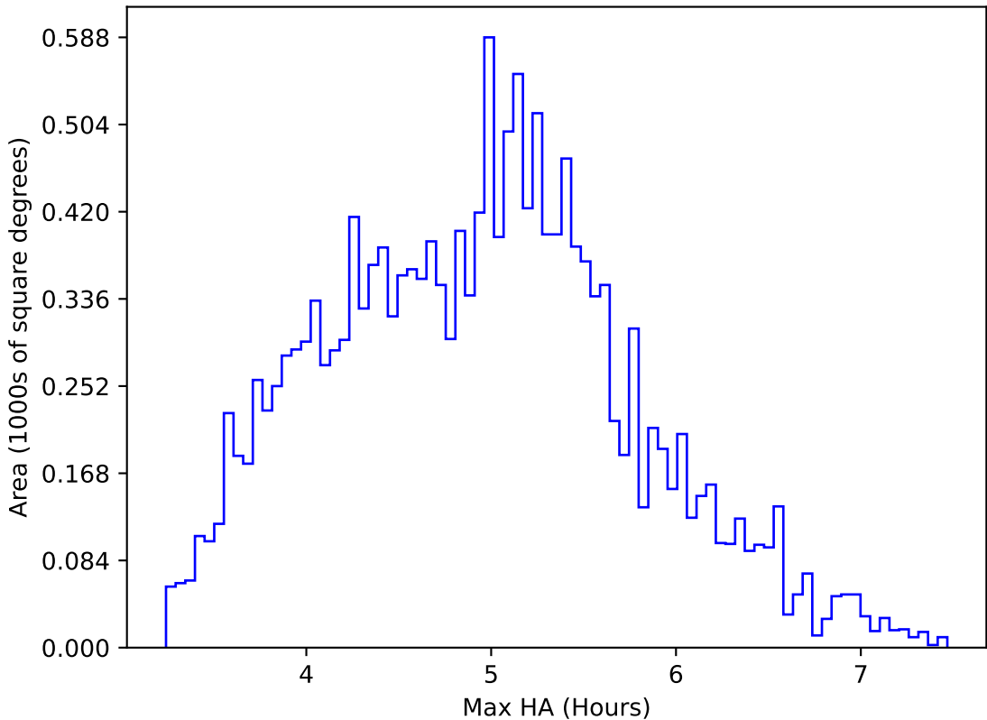
too_elab_heavy_r128_d3_griz_v3.4_10yrs WFD z band: Max HA
