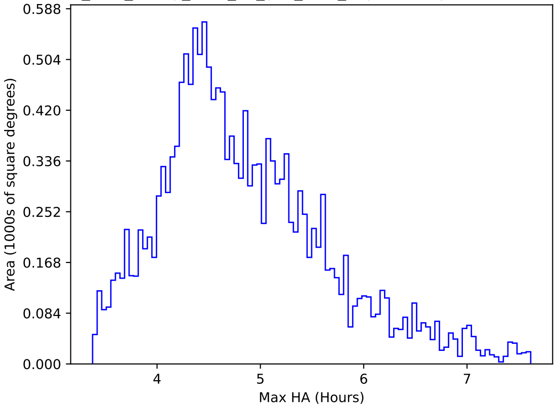
too_elab_heavy_r128_d3_griz_v3.4_10yrs WFD y band: Max HA
