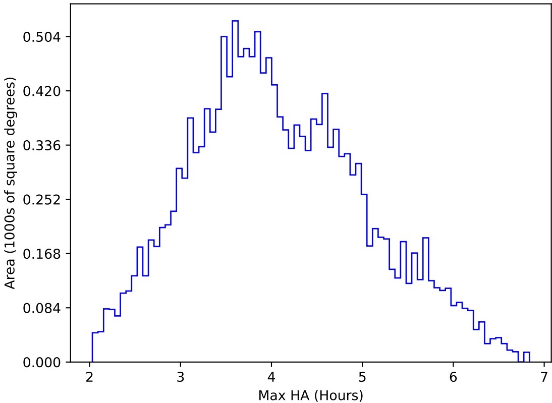
too_elab_heavy_r128_d3_griz_v3.4_10yrs WFD u band: Max HA
