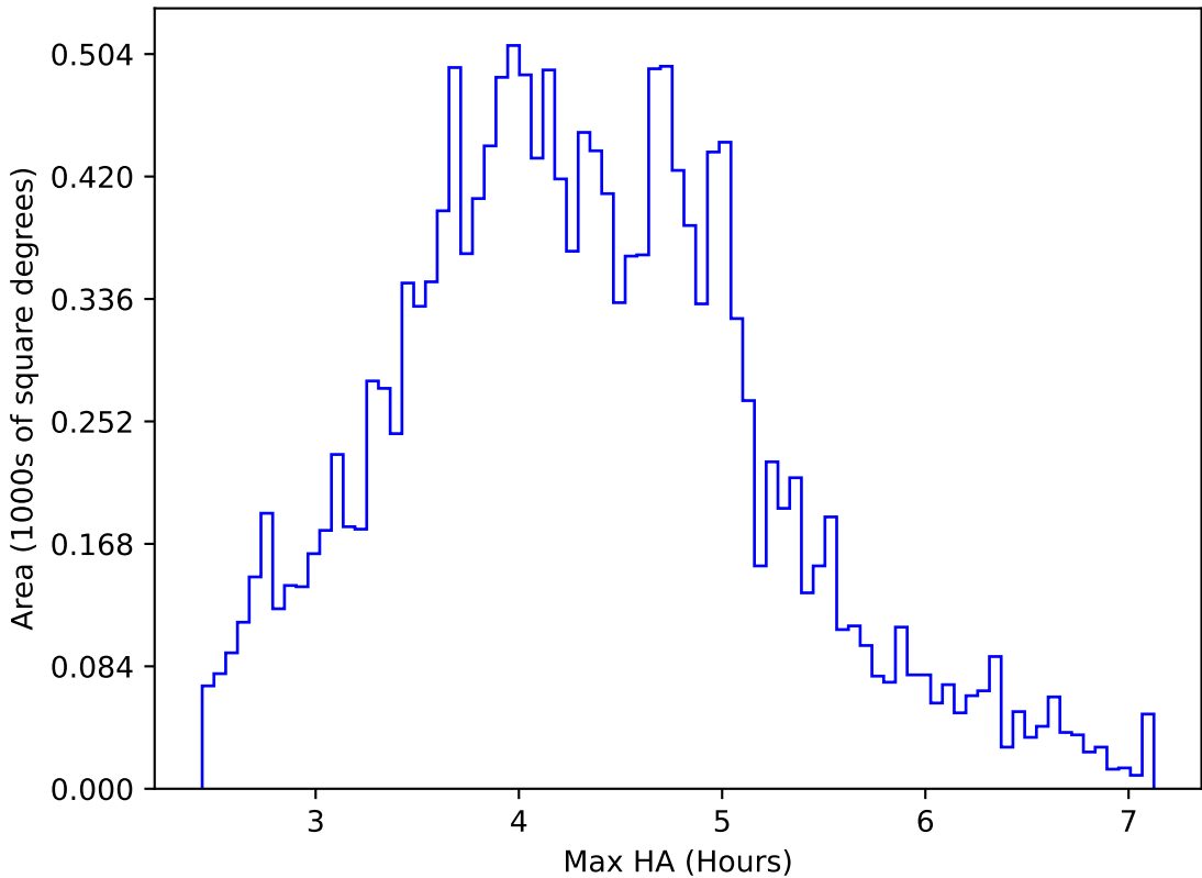
too_elab_heavy_r128_d3_griz_v3.4_10yrs WFD g band: Max HA
