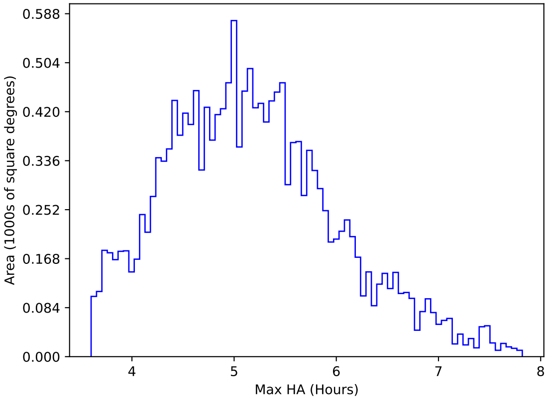
too_elab_heavy_r128_d3_griz_v3.4_10yrs WFD all bands: Max HA
