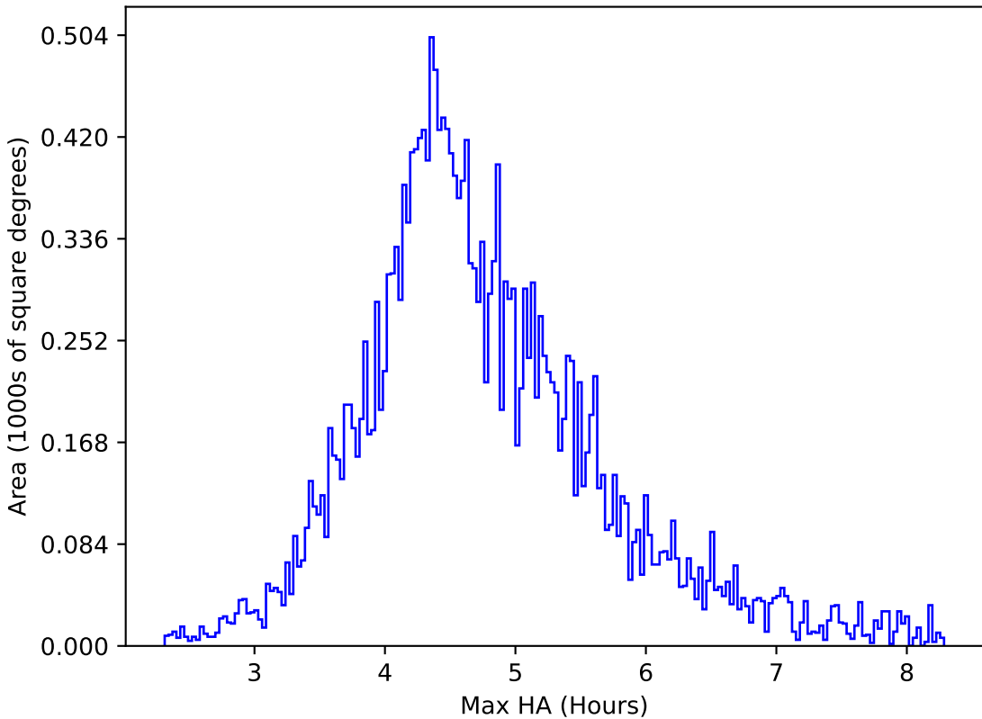
too_elab_heavy_r128_d3_griz_v3.4_10yrs All sky y band: Max HA
