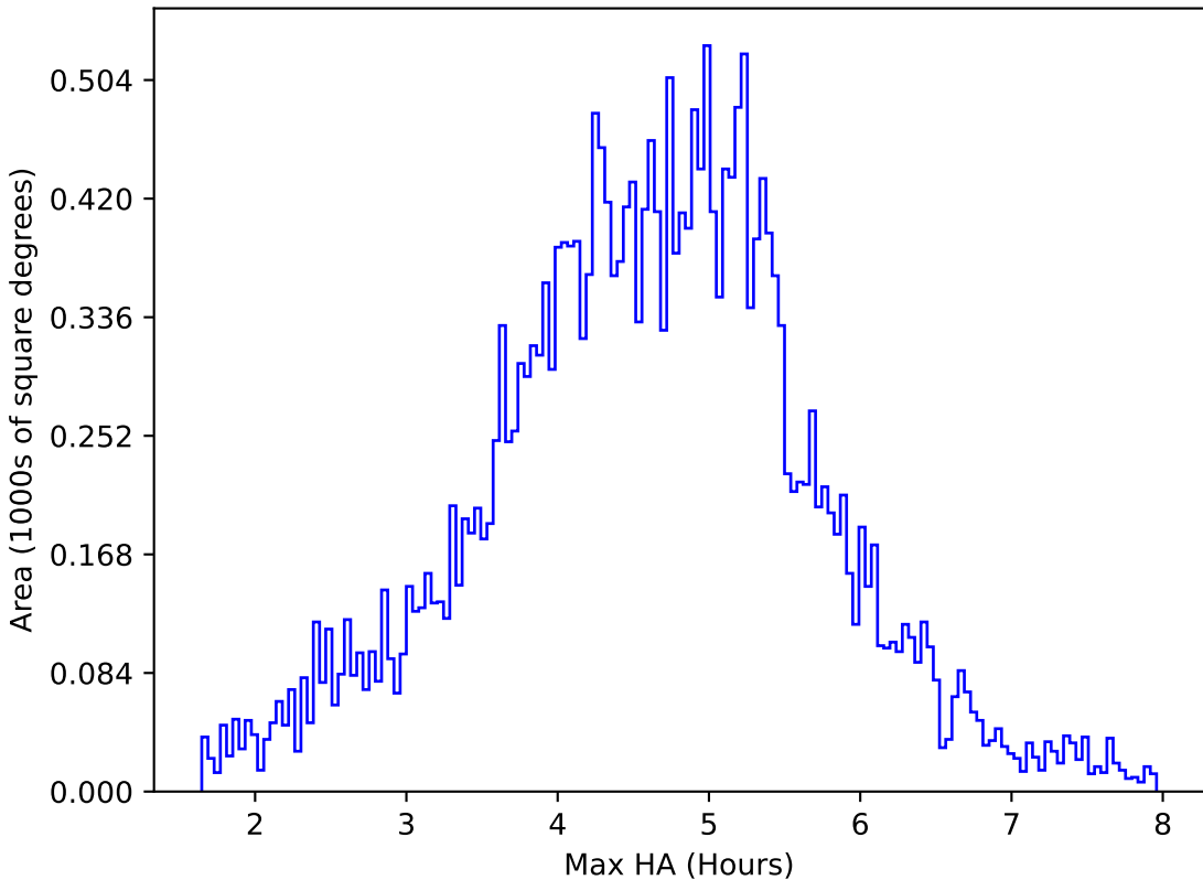
too_elab_heavy_r128_d3_griz_v3.4_10yrs All sky i band: Max HA
