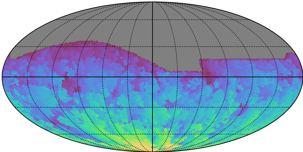
too_elab_heavy_r128_d3_griz_v3.4_10yrs All sky g band: Max HA
