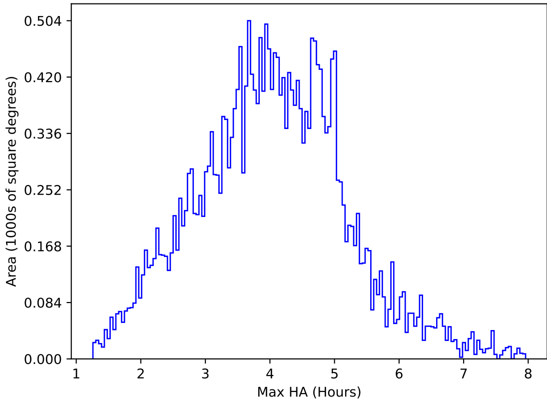
too_elab_heavy_r128_d3_griz_v3.4_10yrs All sky g band: Max HA
