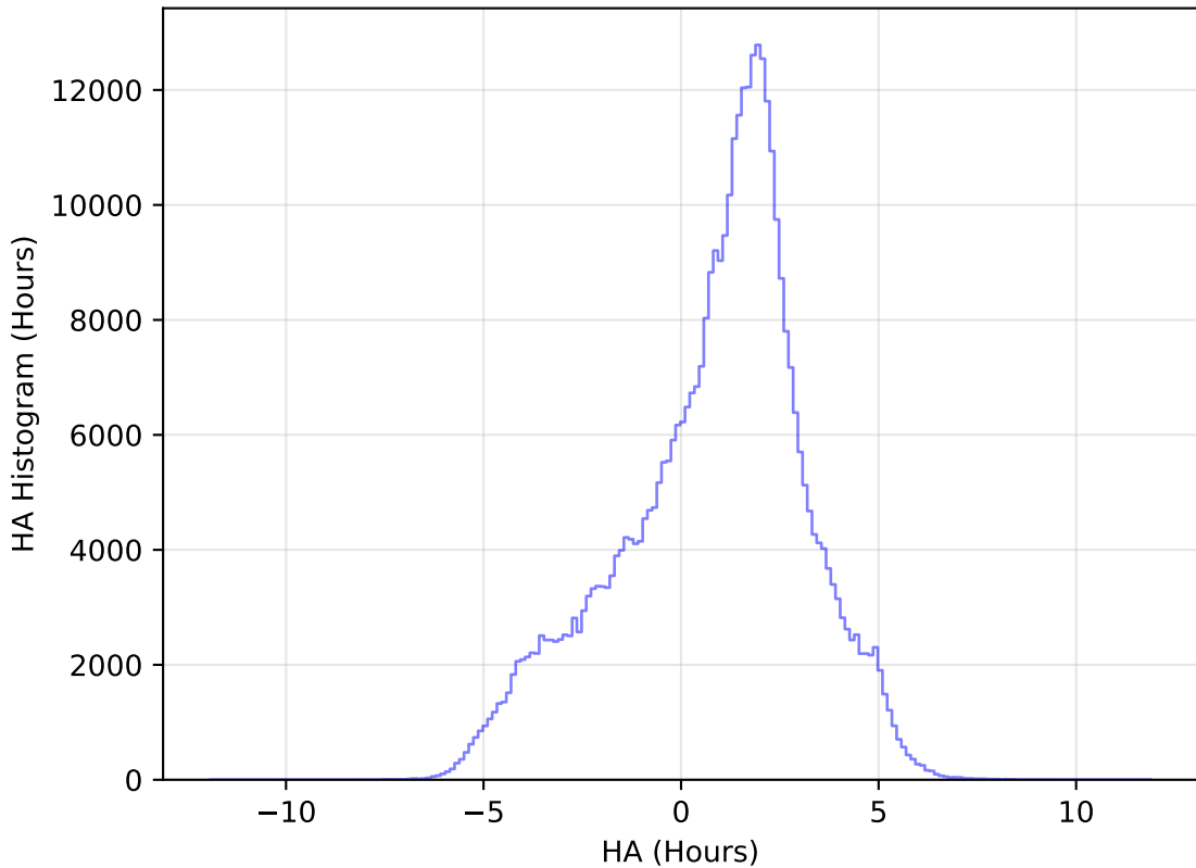
too_elab_heavy_r128_d3_griz_v3.4_10yrs WFD z band: HA Histogram
