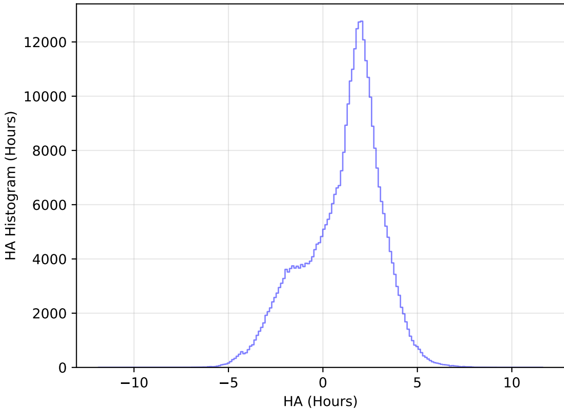
too_elab_heavy_r128_d3_griz_v3.4_10yrs WFD y band: HA Histogram
