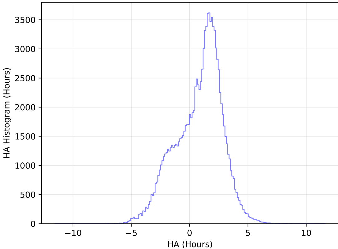
too_elab_heavy_r128_d3_griz_v3.4_10yrs WFD u band: HA Histogram
