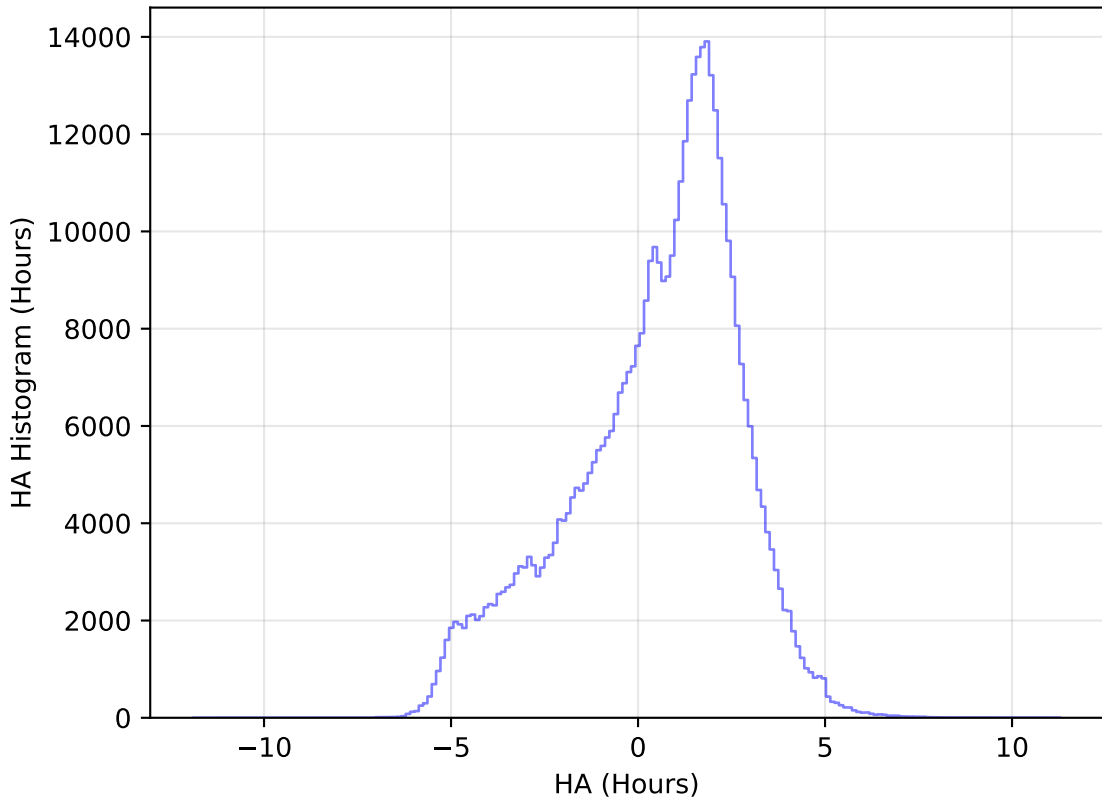
too_elab_heavy_r128_d3_griz_v3.4_10yrs WFD r band: HA Histogram
