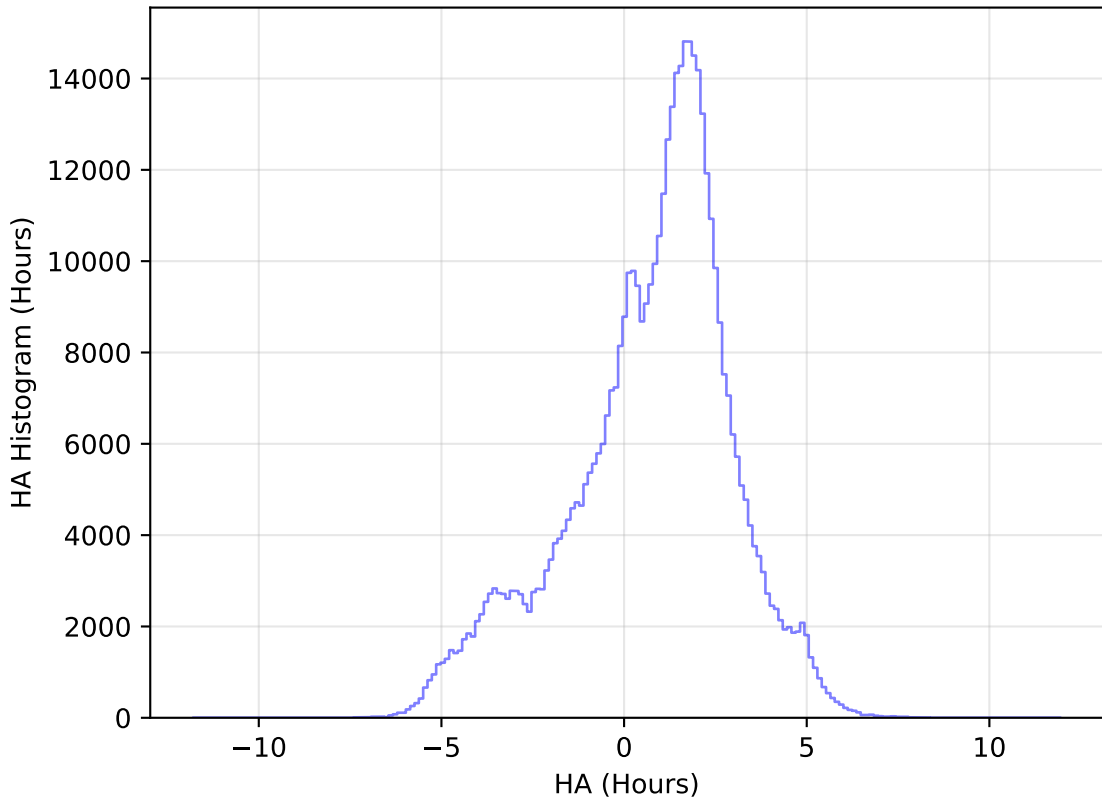
too_elab_heavy_r128_d3_griz_v3.4_10yrs WFD i band: HA Histogram
