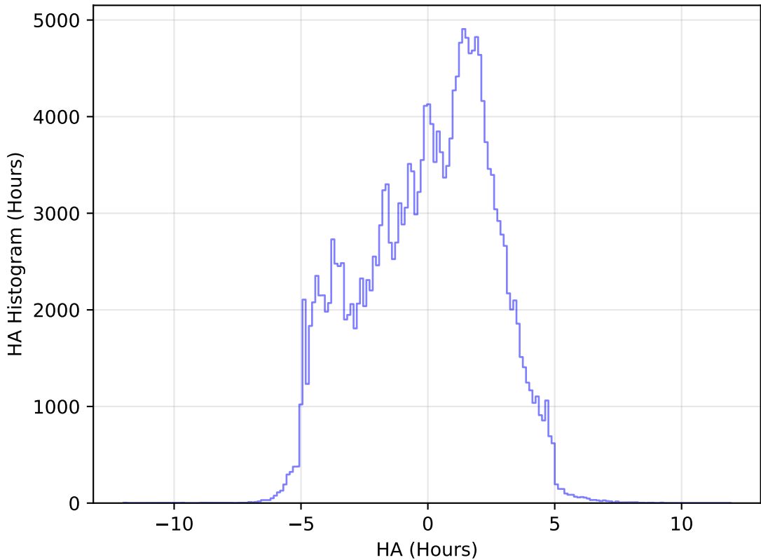
too_elab_heavy_r128_d3_griz_v3.4_10yrs WFD g band: HA Histogram
