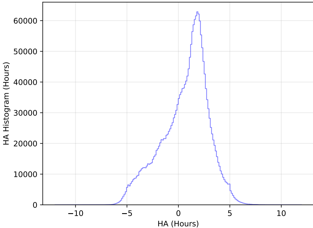
too_elab_heavy_r128_d3_griz_v3.4_10yrs WFD all bands: HA Histogram
