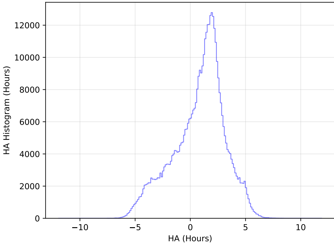
too_elab_heavy_r128_d3_griz_v3.4_10yrs All sky z band: HA Histogram
